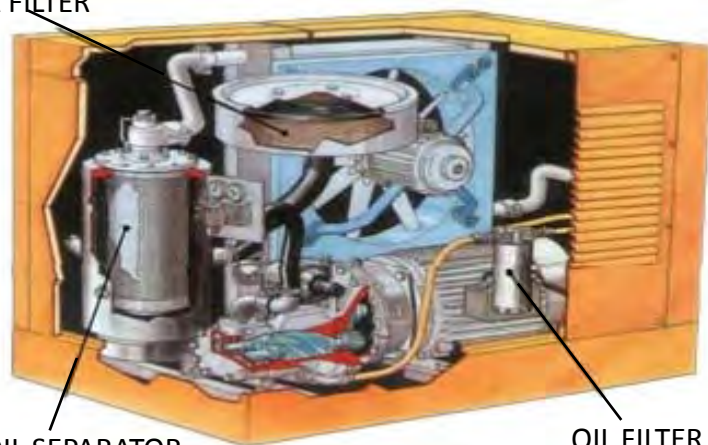
AIR OIL SEPARATOR
